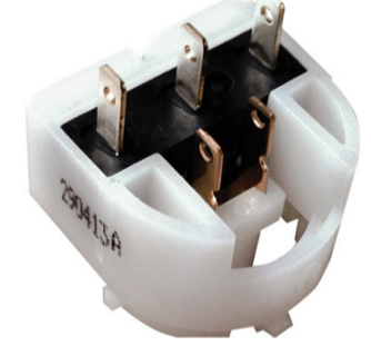
Gamesman Button/ Connector System "U"
