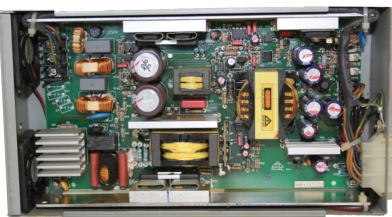
Tri-Mag Power Supply DZ300-12EUFV3 300 Watt
