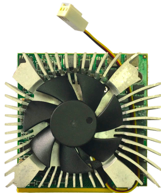
Konami Concerto KP 3.5 Graphics Card MXM-II-E8860 Video Card PT# 106228
