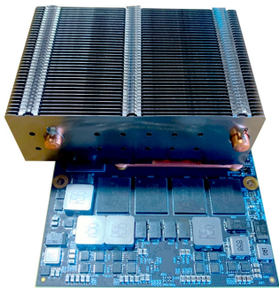
Scientific Games Twinstar Wave XL, J43, E8870 Video Card PT# 106234
