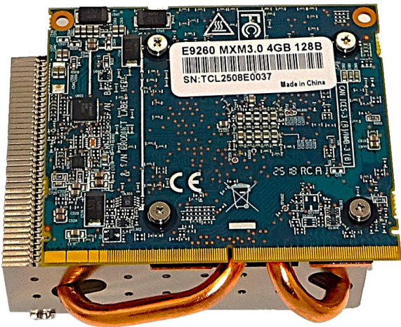
IGT Crystal E9260 MXM 3.0 Video Card
