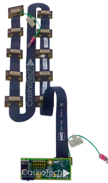
Ribbon Cable for IGT Edge Lit and Non Edge Lit Button Panel PT# 100334
