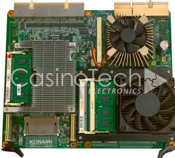
KP3.5 Concerto CPU MXM-II E8860 PT# 104510
