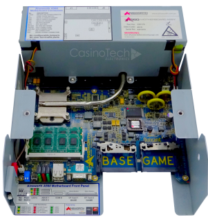
Ainsworth A560 Assembly PT# 104522
